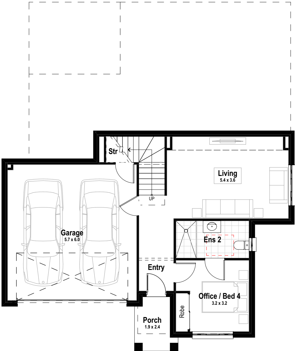
GROUND FLOOR
