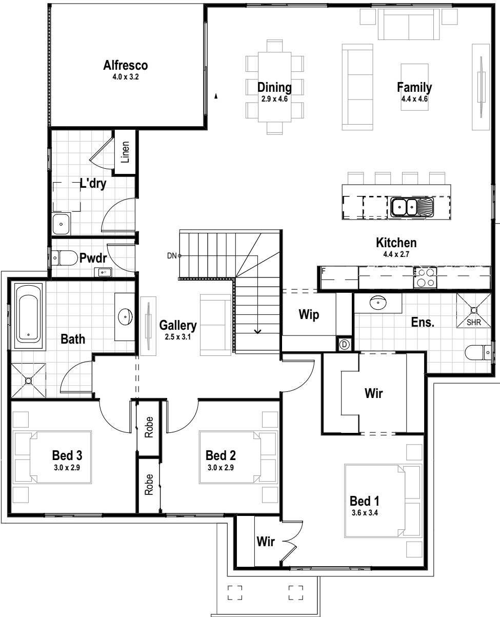
FIRST FLOOR
